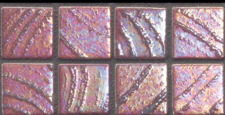
Mauna Loa
