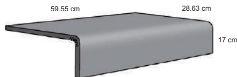
▲ STEP L 60° 28,63 x 59,55 x 17 cm
